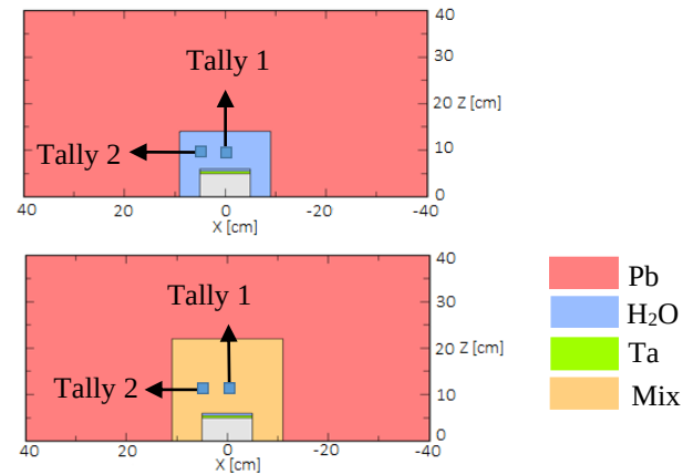
Fig. 1. Geometry model for the water moderator (upper) and mixture moderator (below).
